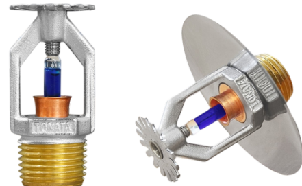
TNT-SPP141 SPRINKLER PENDENT 141C
